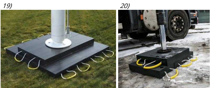
Fig. 17: Single crane support plate Fig. 18: Crane support plates stacked Fig. 19+20: Application examples
